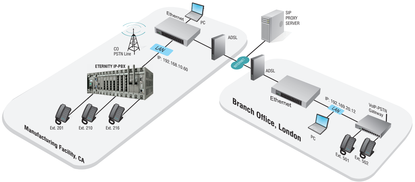
Figure 4: Multi-site Connectivity over IP Intra - office cost saving through Peer -to- Peer Calling
